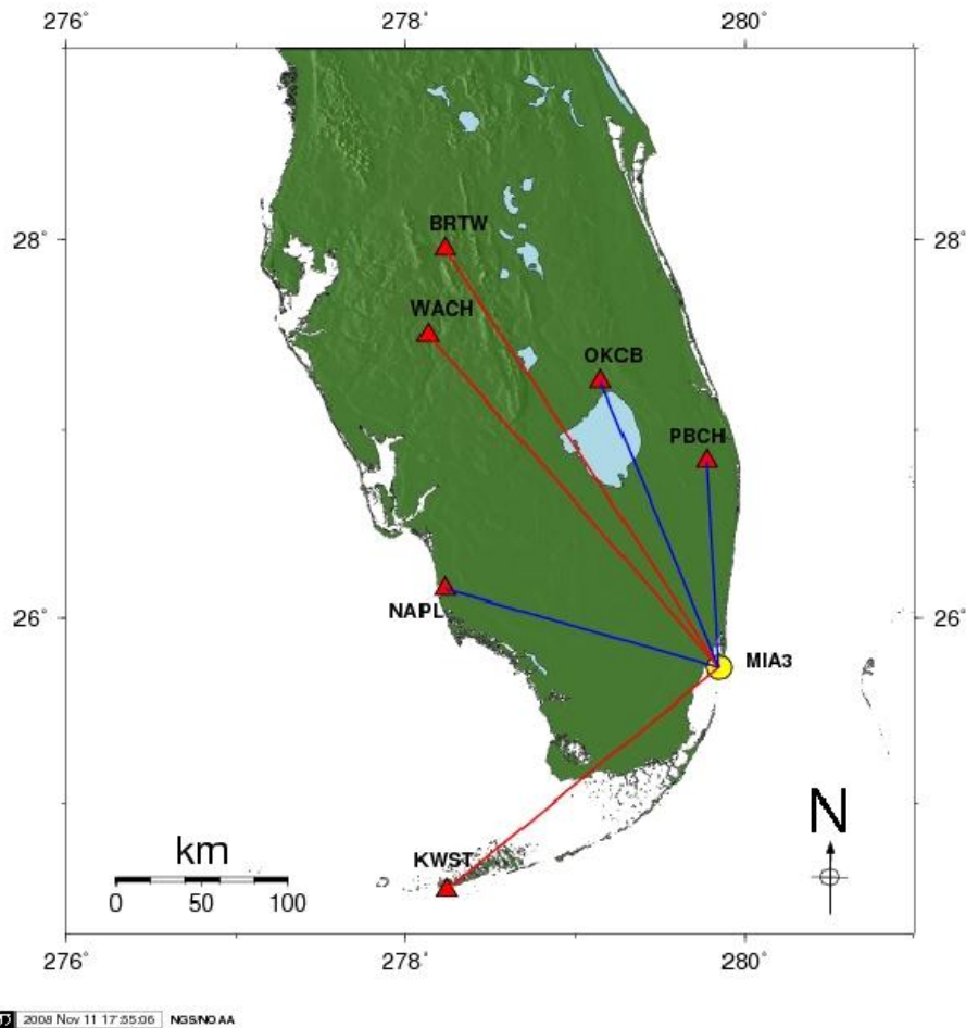
Fig. 4. Reference station selection by OPUS based on constraining baseline ranges. Reference stations connected with blue baselines were chosen when 100-200 km was the constraining range while red baselines connect reference stations 200-300 km away.
