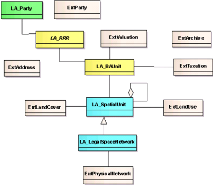
Figure 2. LADM and external classes
