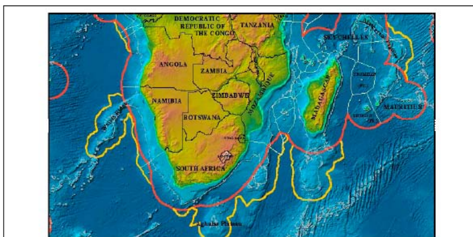
Figure 6 - Hypothetical extension of the continental shelf beyond 200 M for southern Africa (shown in orange).
