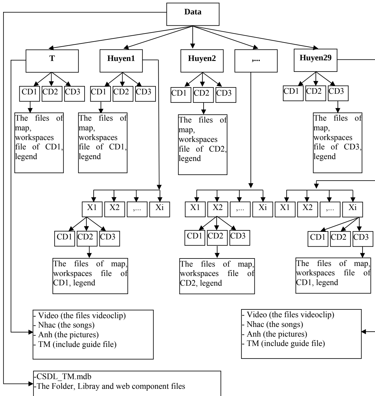
Fig. 2: The diagram of data stored in the Atlas.
