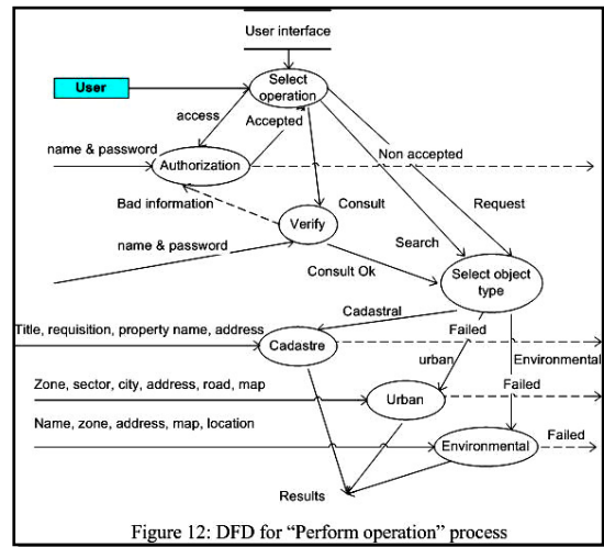
Figure 12: DFD for “Perform operation” process
