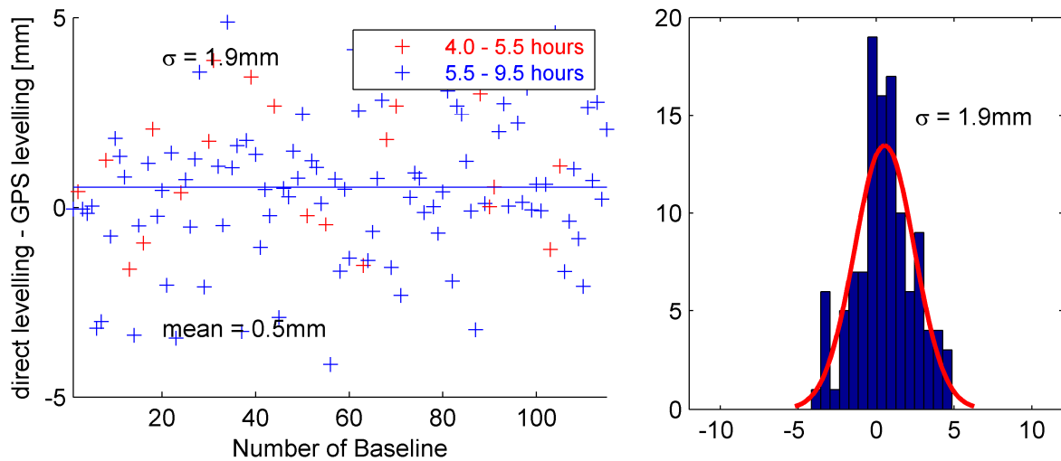
Fig. 7: Differences between GPS and precise leveling (L2)
