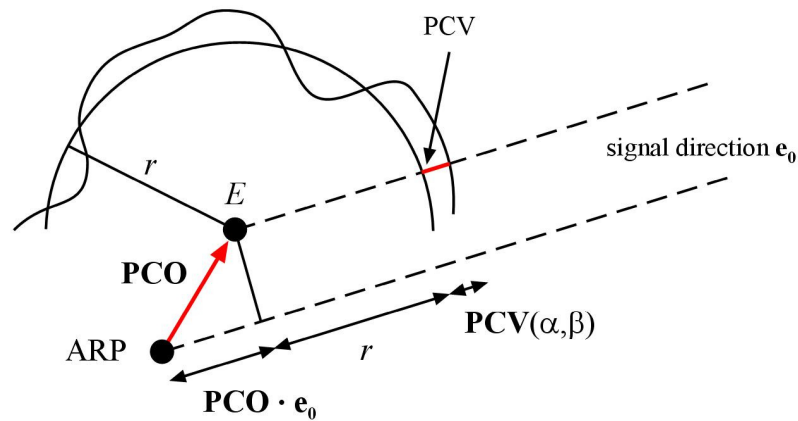
Fig. 1: Antenna model ( Zeimetz and Kuhlmann 2008 ).
