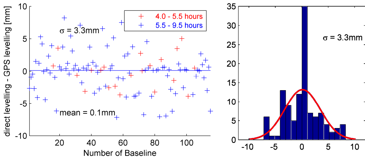
Fig. 8: Differences between GPS and precise leveling (L0)
