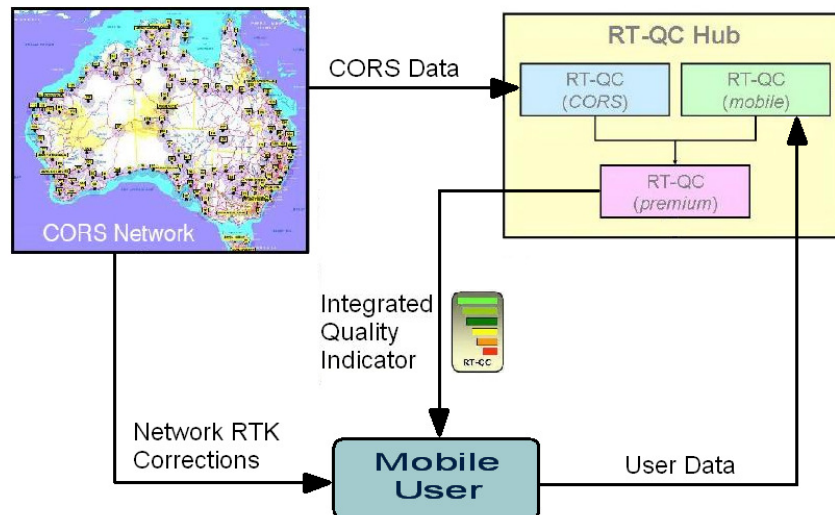
Figure 3. RTQC Mobile Setup
