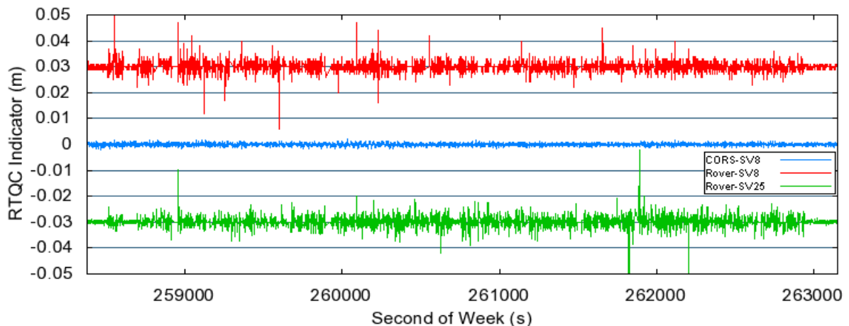
Figure 7. Individual RTQC Indicators during railway survey on 4 th March 2009.
