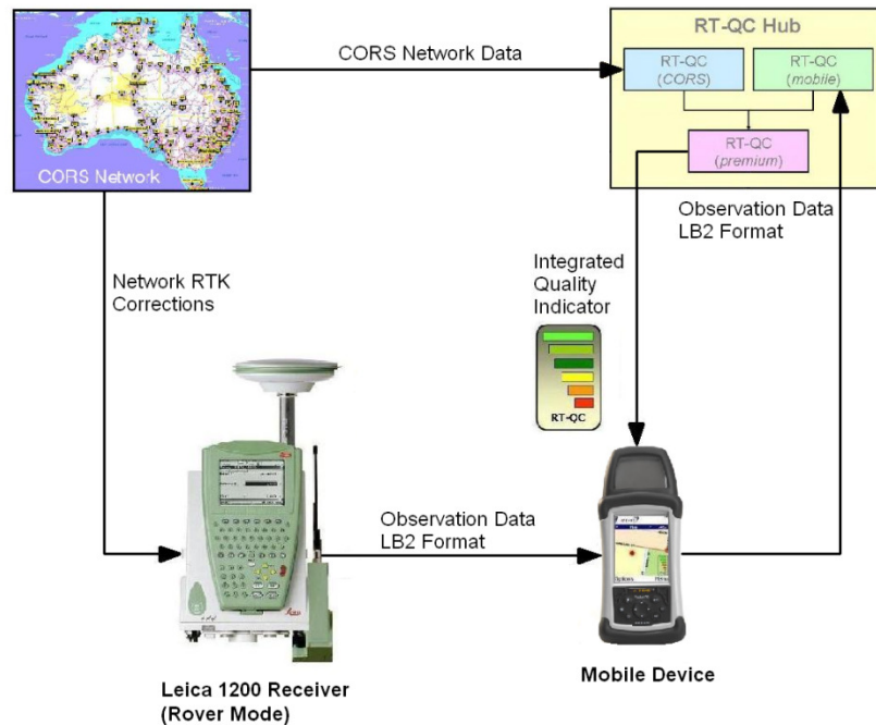
Figure 5. Leica Rover Set Up.
