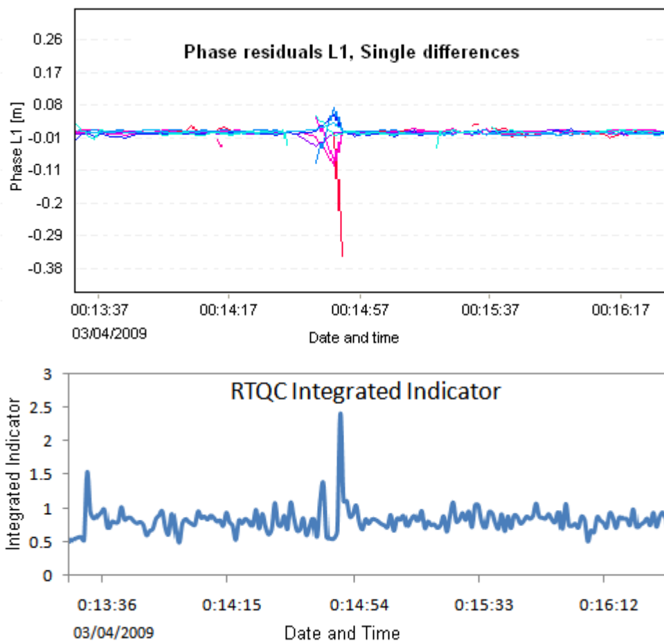
Figure 9. L1 Phase residuals and RTQC Integrated Indicator
