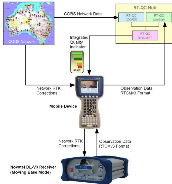
Figure 4. Novatel Moving Base Set Up.
