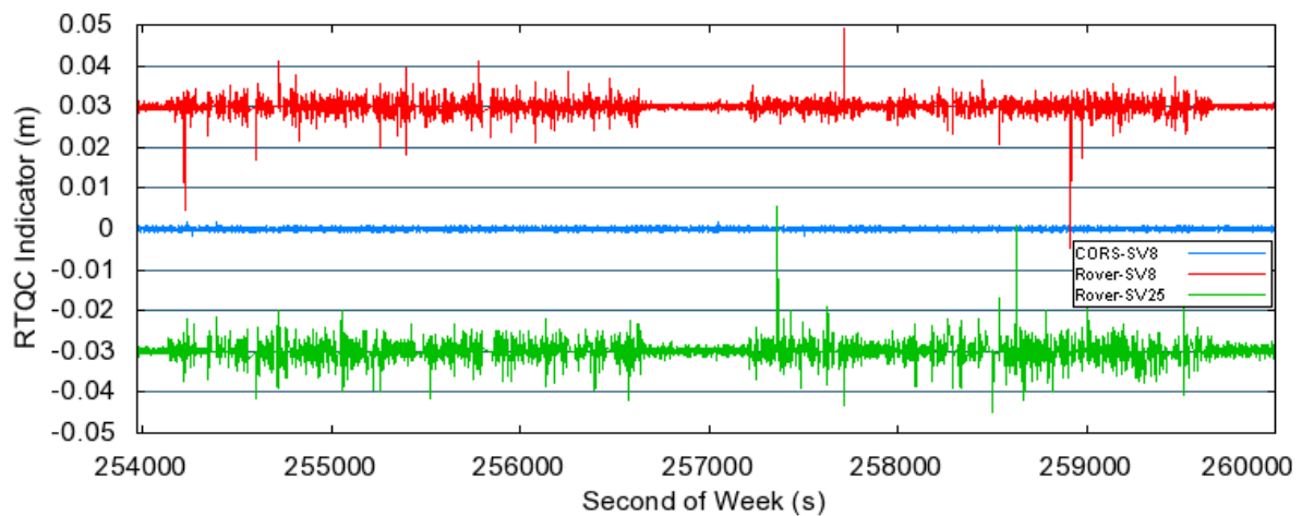
Figure 8. Individual RTQC Indicators during railway survey on 1 st April 2009.
