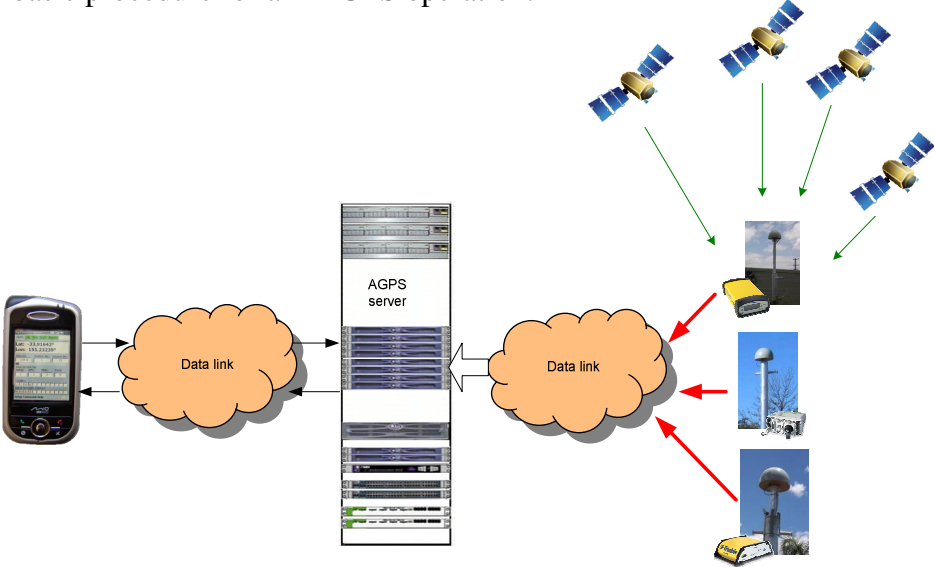
Figure 2. The general technique of A-GPS.
