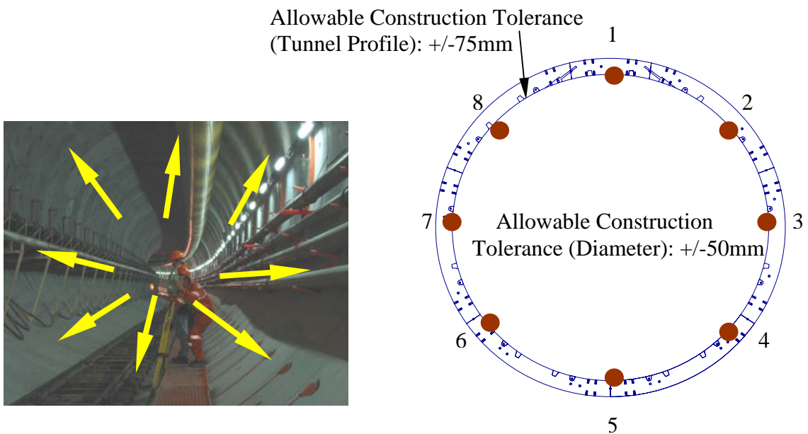
Figure 22 A standard eight point wriggle survey
