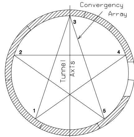
Figure 27 Convergence array
