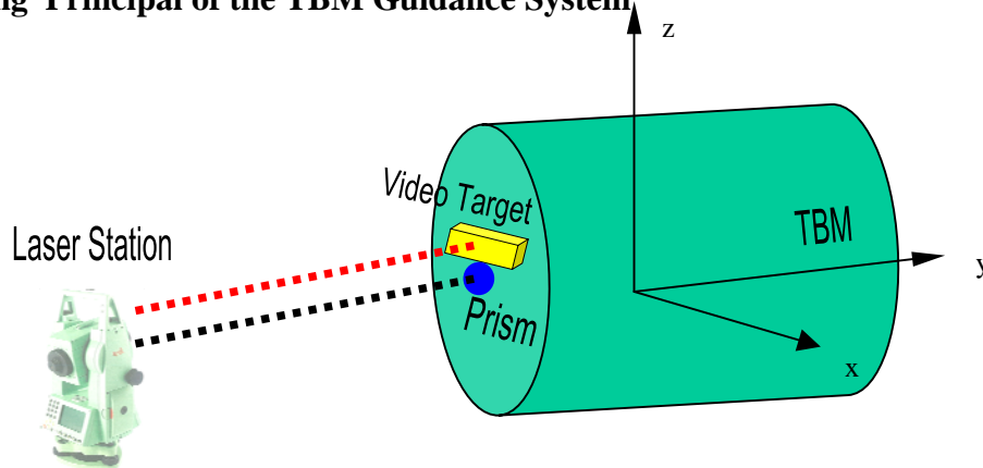
Figure 11 The Laser Station of the TBM Guidance System
