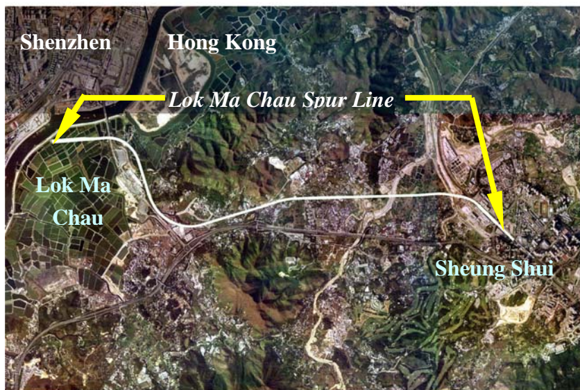
Figure 3 The Lok Ma Chau Spur Line
