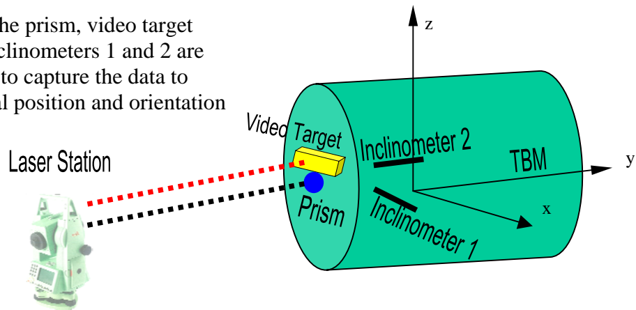
Figure 15 The mechanism of data acquisition of the tunnel guidance system
