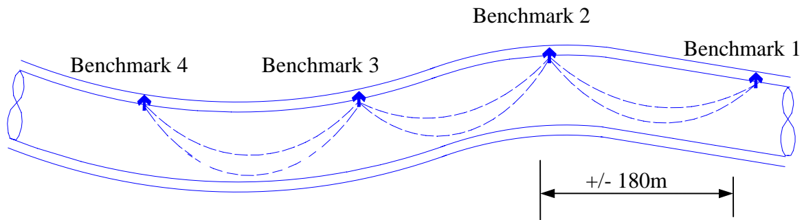
Figure 26 Benchmark looping
