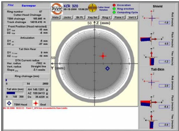
Figure 18 The screen display of the travelling TBM and its deviation from the design path.
