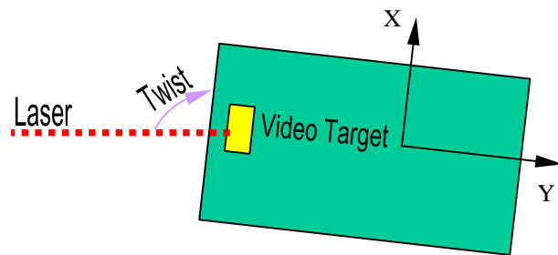
Figure 12 Plan View
