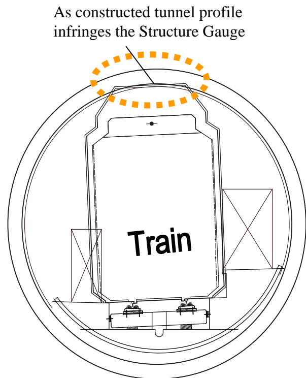
Figure 24 Infringement of the structural gauge of the train
