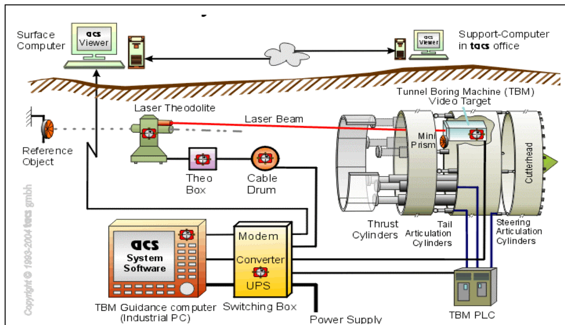
Figure 16 Processing of captured data of the moving TBM
