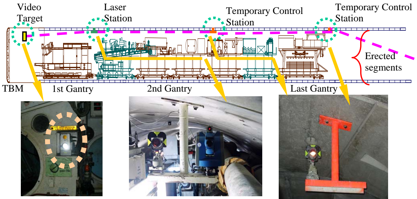
Figure 10 Transfer of control station at the TBM back up gantry
