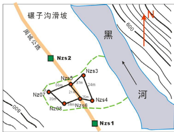
Fig 8. The monitored landslide over a reservoir
