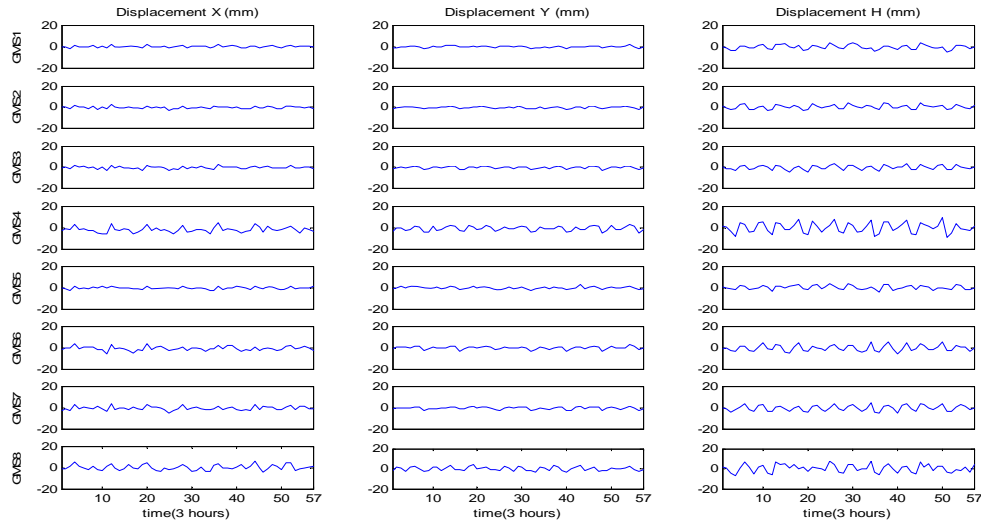
Fig 12. Displacement series with 3 hour data update interval
