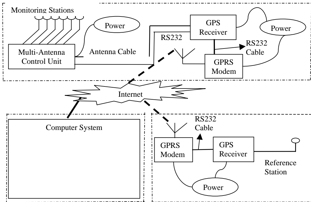
Fig 1. Multi-antenna GPS system structure
