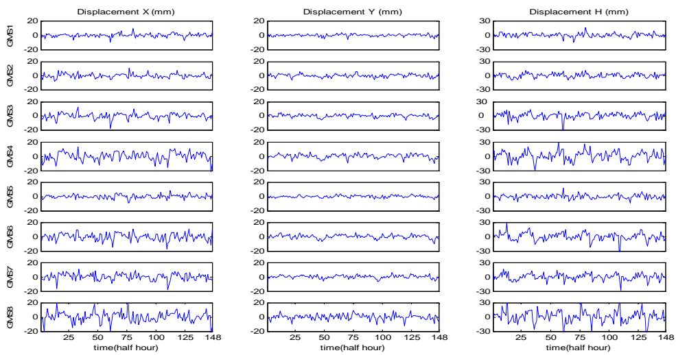
Fig 10. Displacement series in with 30 minute data update interval
