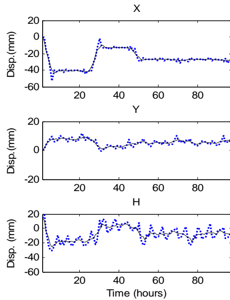
Fig7. The measured displacement series
