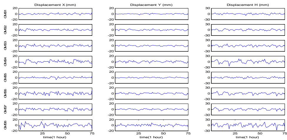
Fig 11. Displacement series with 1 hour data update interval
