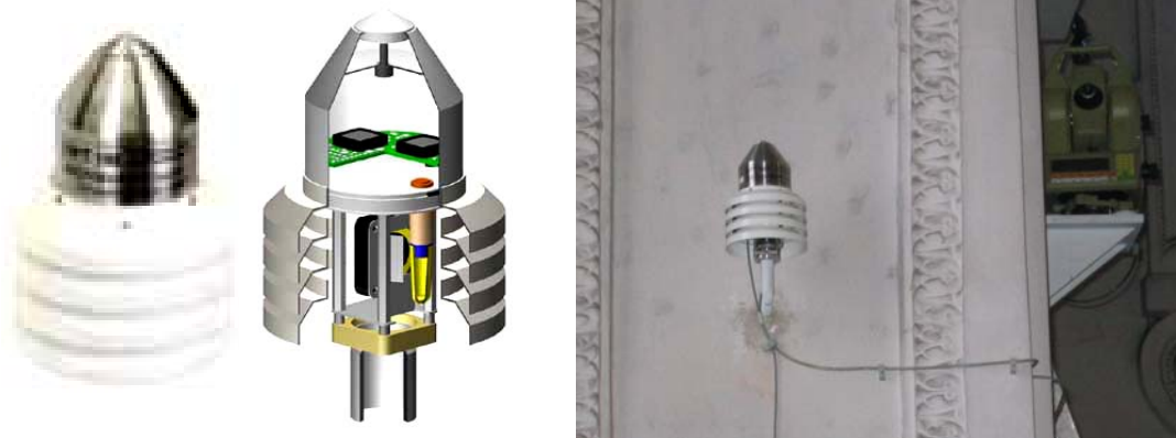
Figure 4: Sensors: Reinhardt DMT 1MV (left) and Leica-TCA2003 (right)
