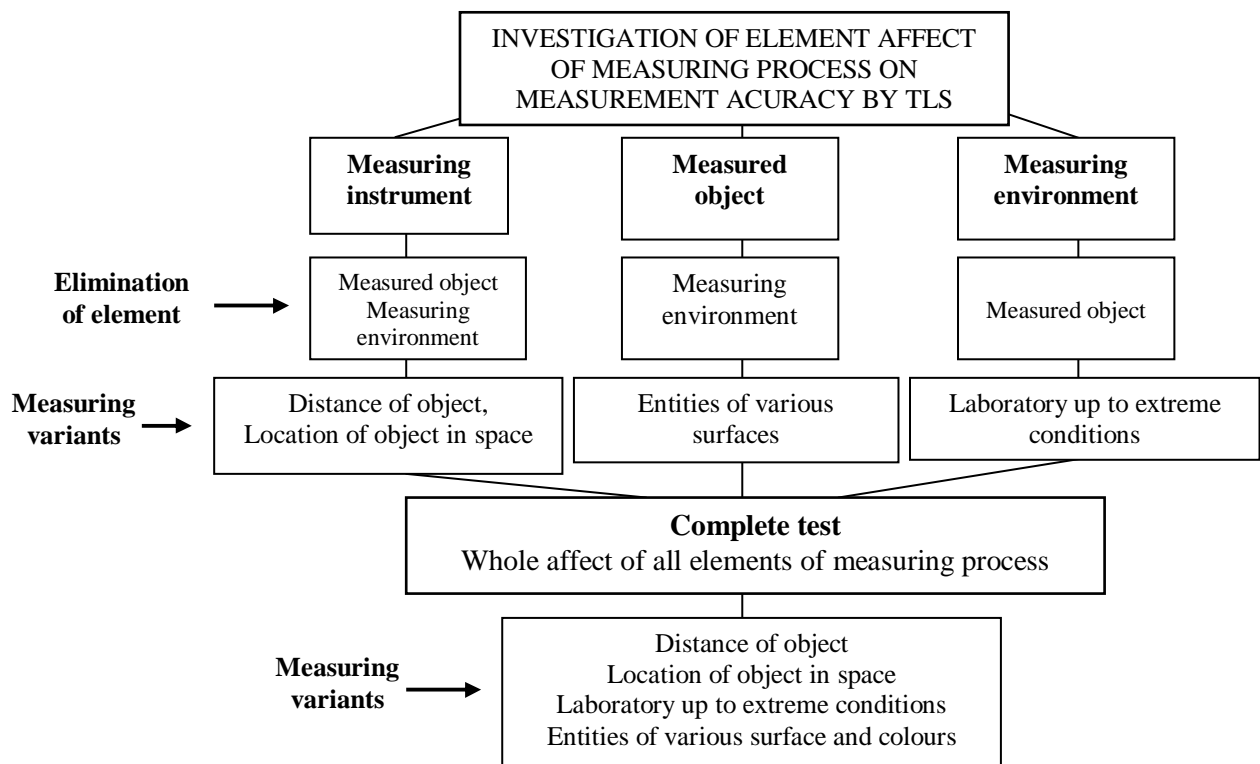
Fig. 3: Measurement variants for investigation of elements affect of measuring process at measuring accuracy
