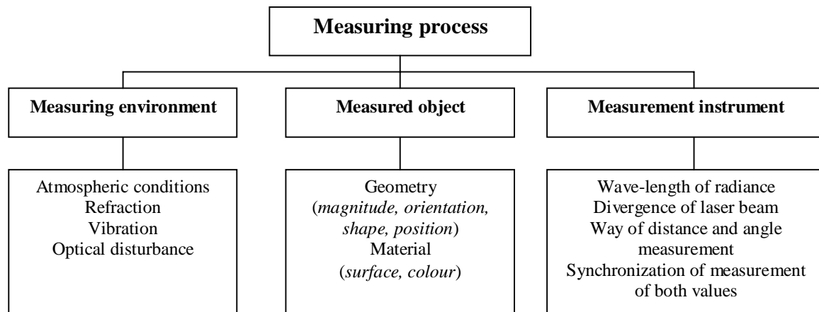
Fig. 2: Element properties of measurement process
