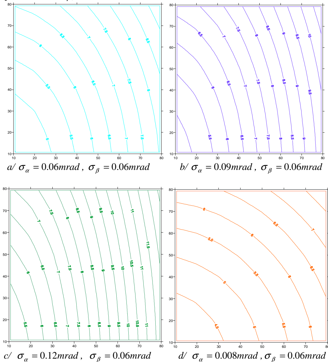
Fig. 1: Graphical presentation of \sigma_p isolines by X-coordinate fixed
