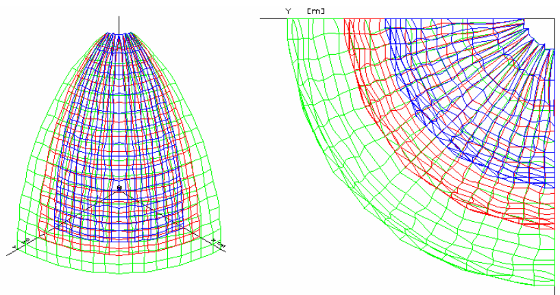
Fig.3: Surfaces with the same uncertainty in point position – Microstation SE software -green \sigma_{\alpha}=0.06\text{mrad} , \sigma_{\beta}=0.06 \text{ mrad} - red \sigma_{\alpha}=0.09\text{mrad} , \sigma_{\beta}=0.06 \text{ mrad} - blue \sigma_{\alpha}=0.12\text{mrad} , \sigma_{\beta}=0.06 \text{ mrad}
