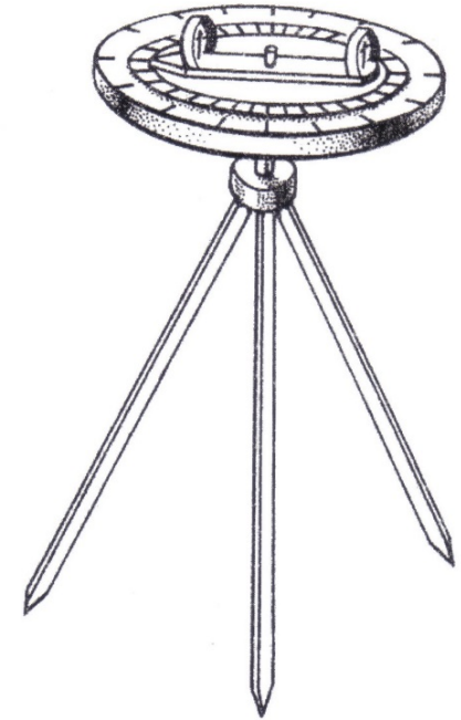
Dioptra. Draft by Heron.
