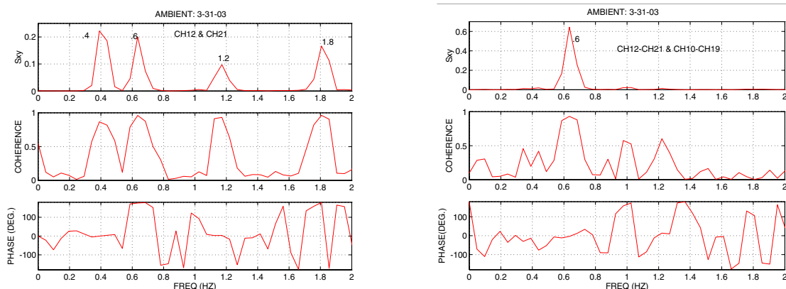
Fig. 6. Cross-spectrum, coherency, and phase angle plots of ambient acceleration response data obtained from (a-left) parallel channels (CH12 and CH21) at the roof and (b-right) differences of parallel channels, CH12 - CH21 at the roof and CH10-CH19 at the 18 th floor.
