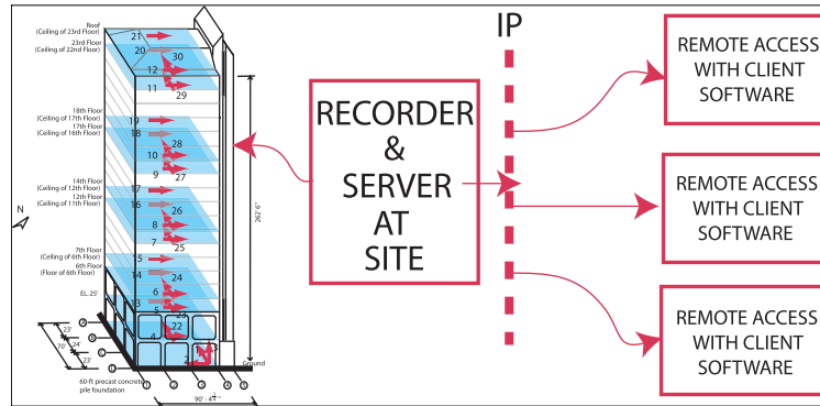
Fig. 3. General schematic of data acquisition and transmittal for seismic monitoring of the building.
