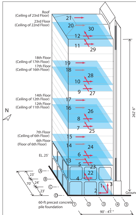
Fig. 1. General three-dimensional schematic of the building. Also shown are the 30 accelerometers (heavy arrows) deployed throughout the building.
