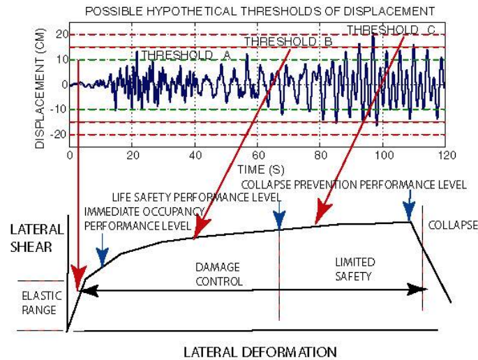
Fig. 2. Hypothetical displacement time-history as related to FEMA 274.
