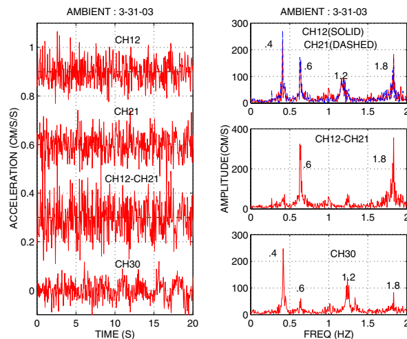
Fig. 5. Twenty seconds of ambient acceleration response data obtained at the roof from parallel channels (CH12 & CH21), their difference (CH12-CH21), and from CH30, orthogonal to CH12 and CH21 (left) and corresponding amplitude spectra (right).
