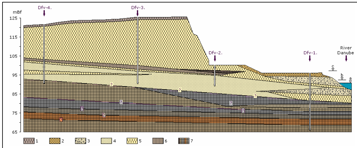
Figure 6: Geological cross-section between Felső-Öreghegy and the river Danube on the basis of the geotechnical survey performed by Pyrus Ltd. in 1994. Legend: 1 – recent filling mixed with silt affected by pedogenesis, 2 – sandy, pebbly filling, 3 – sandy gravel, 4 – sand, 5 – typical loess, 6 – palaeosol, 7 – clay, Dfv-1. –Dfv-4.: exploratory drillings, a – LW (lowest water), b – AW (average water), c – HW (highest water)
