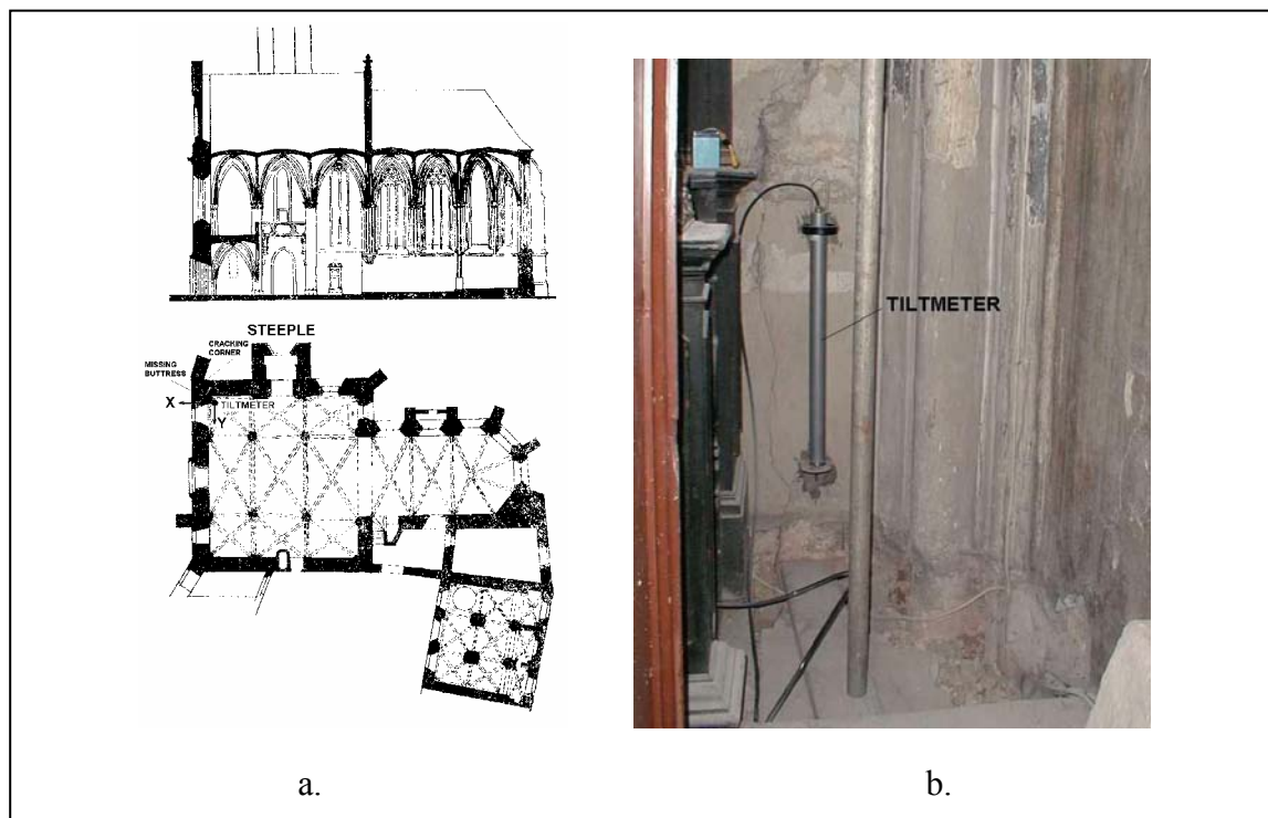
Figure 5: Installation of the tiltmeter in the Church Kecske
