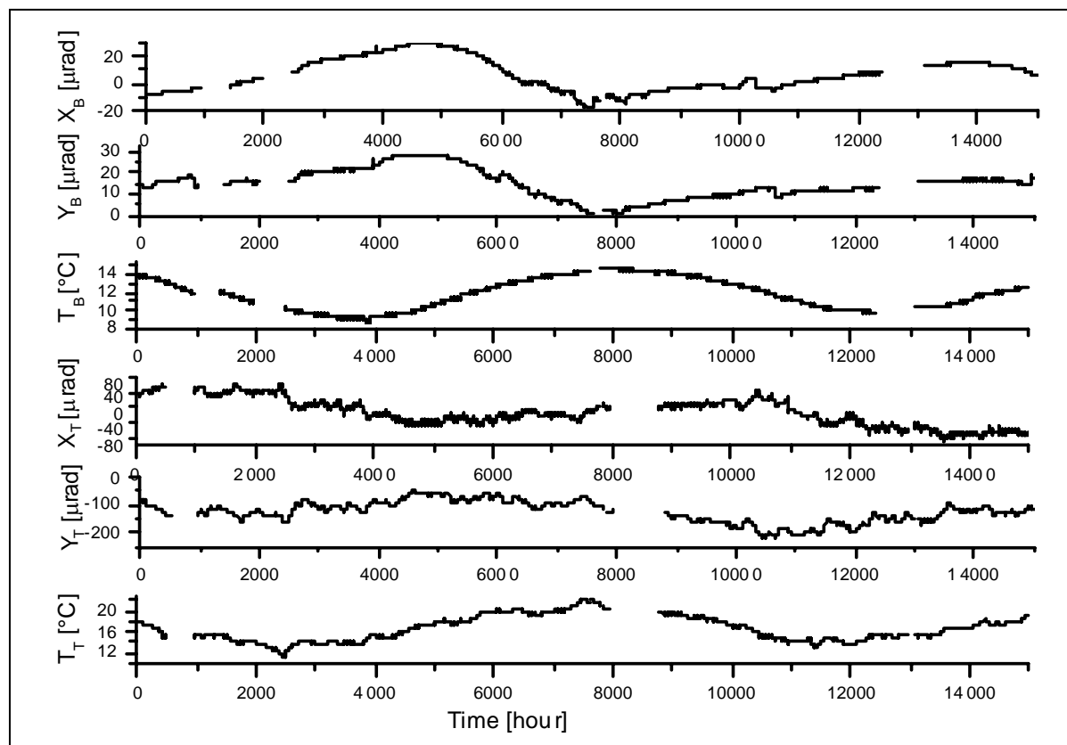
Figure 3: Raw data recorded at the TV tower from 11.04.1999 to 05.07.2001
