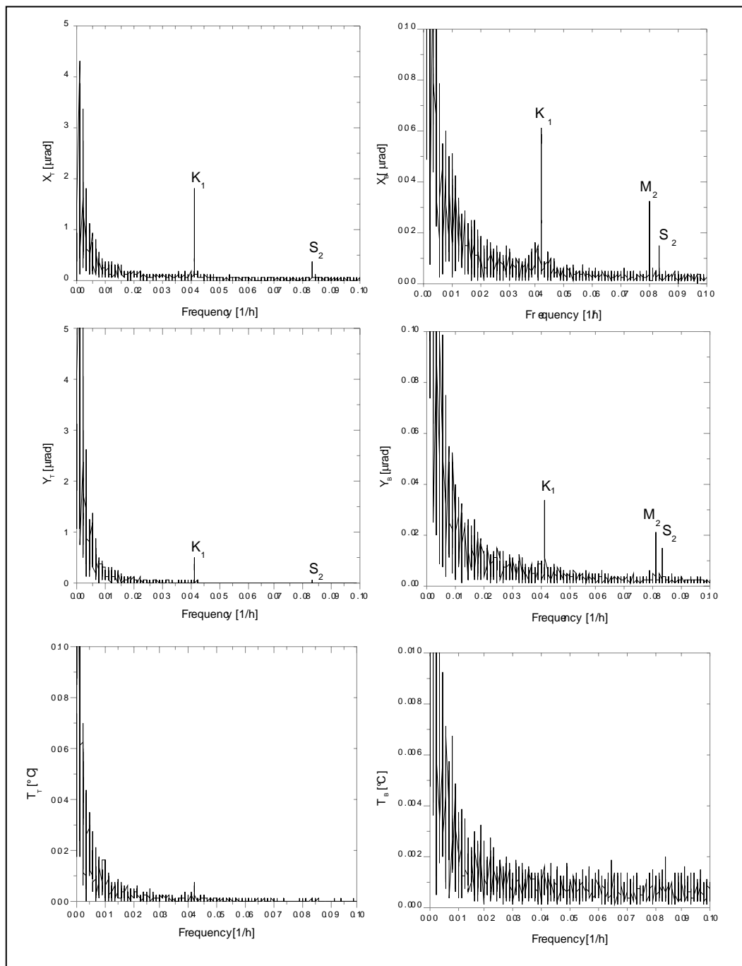
Figure 4: Amplitude spectra of the residual signals
