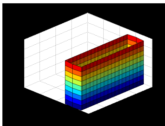
Figure 3: A Three-dimension Analytic Building Model with Equation (2), where z_{h_{\min}}^{h_{\max}} = 0
